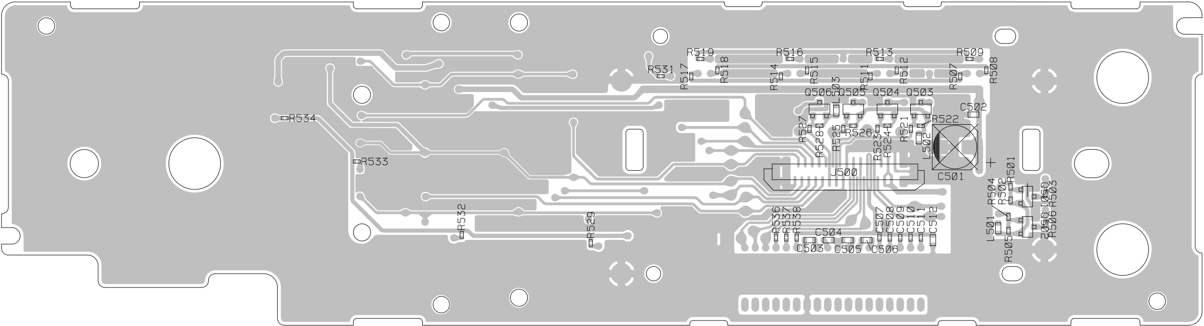
B501: PH-314BA 1/5 (BOTTOM VIEW)
