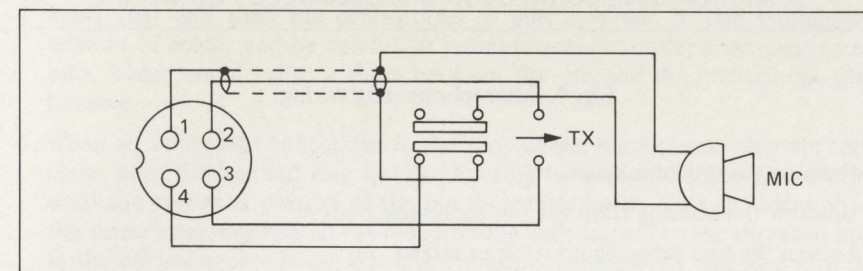
Fig. 3. SUPER STAR 360 FM microphone schematic.
