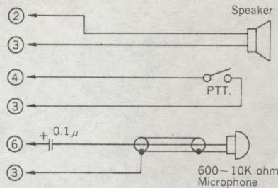
2. Headset or Telephoneset with PTT.
