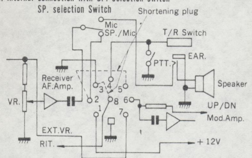
8. Internal connection with SP. selection switch
