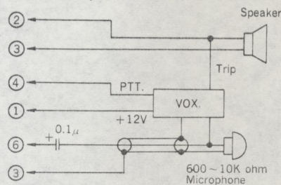
4. Headset or Telephoneset with VOX.
