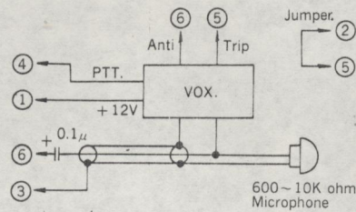
2. Headset or Telephoneset with PTT.
