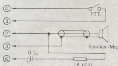
5. External Microphone Speaker with PTT.
