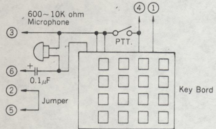
6. Telephone encoder Mic.
