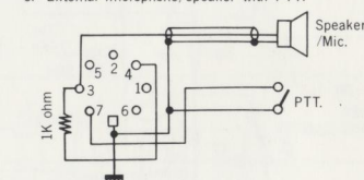
5. External microphone/speaker with PTT.
