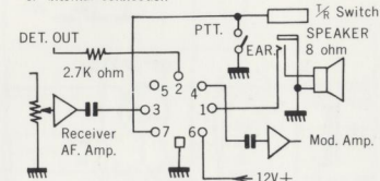
6. Internal connection
