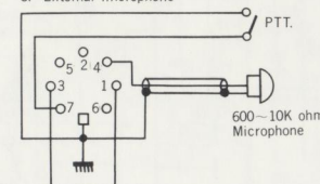
3. External microphone
