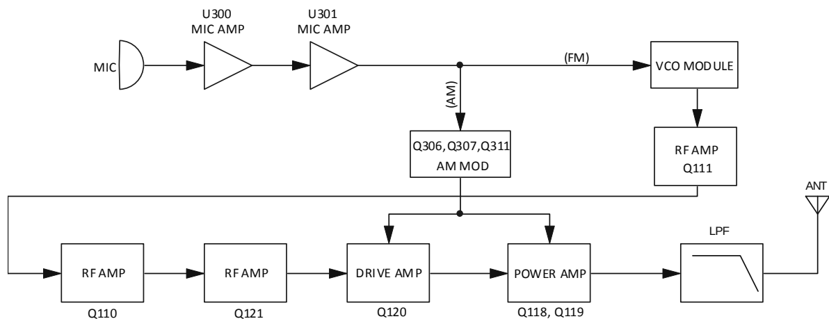
Fig. 5 Transmit circuit
