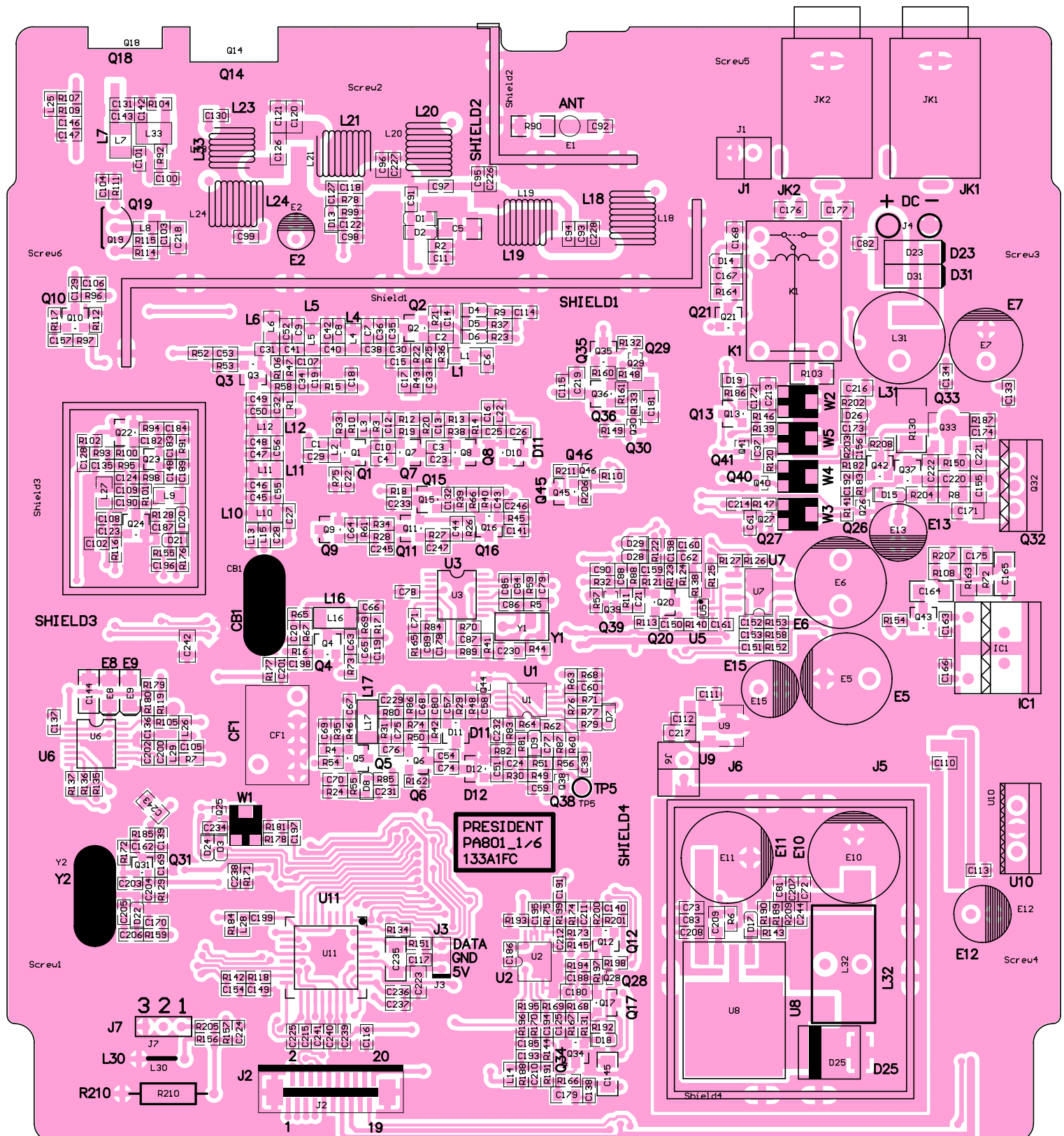
PRESIDENT ANDY AM/FM Main PCB component layout 20 12 2016
