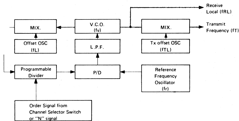
Fig. 5 Theoretical Block Diagram of PLL Frequency Synthesizer Circuitry for CB transceiver
