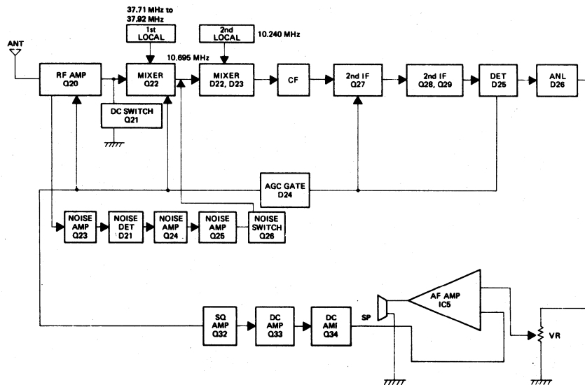
Fig. 8 AM RECEIVER
