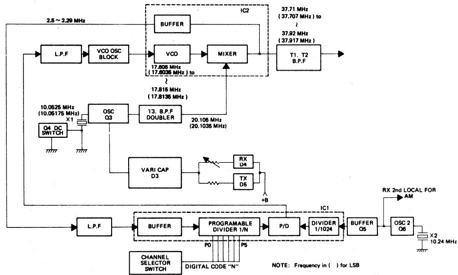
Fig. 7 PLL CIRCUIT
