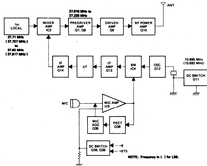
Fig. 11 SSB TRANSMITTER
