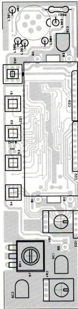
COMPONENT SIDE
