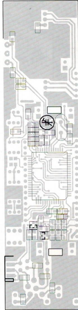
COMPONENT SIDE
