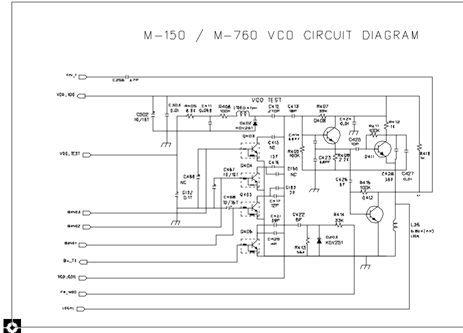
VCO CIRCUIT DIAGRAM
