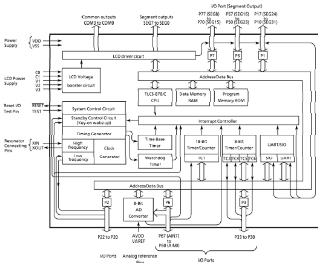
Block Diagram
