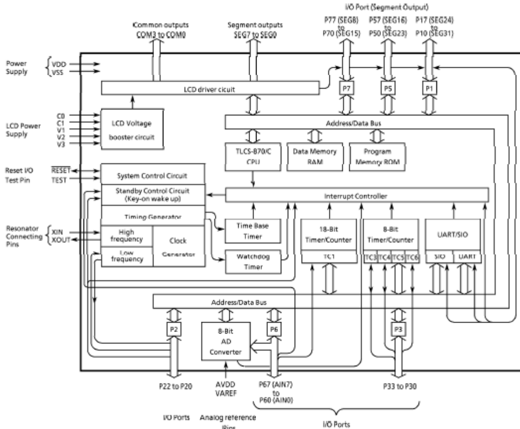
Block Diagram
