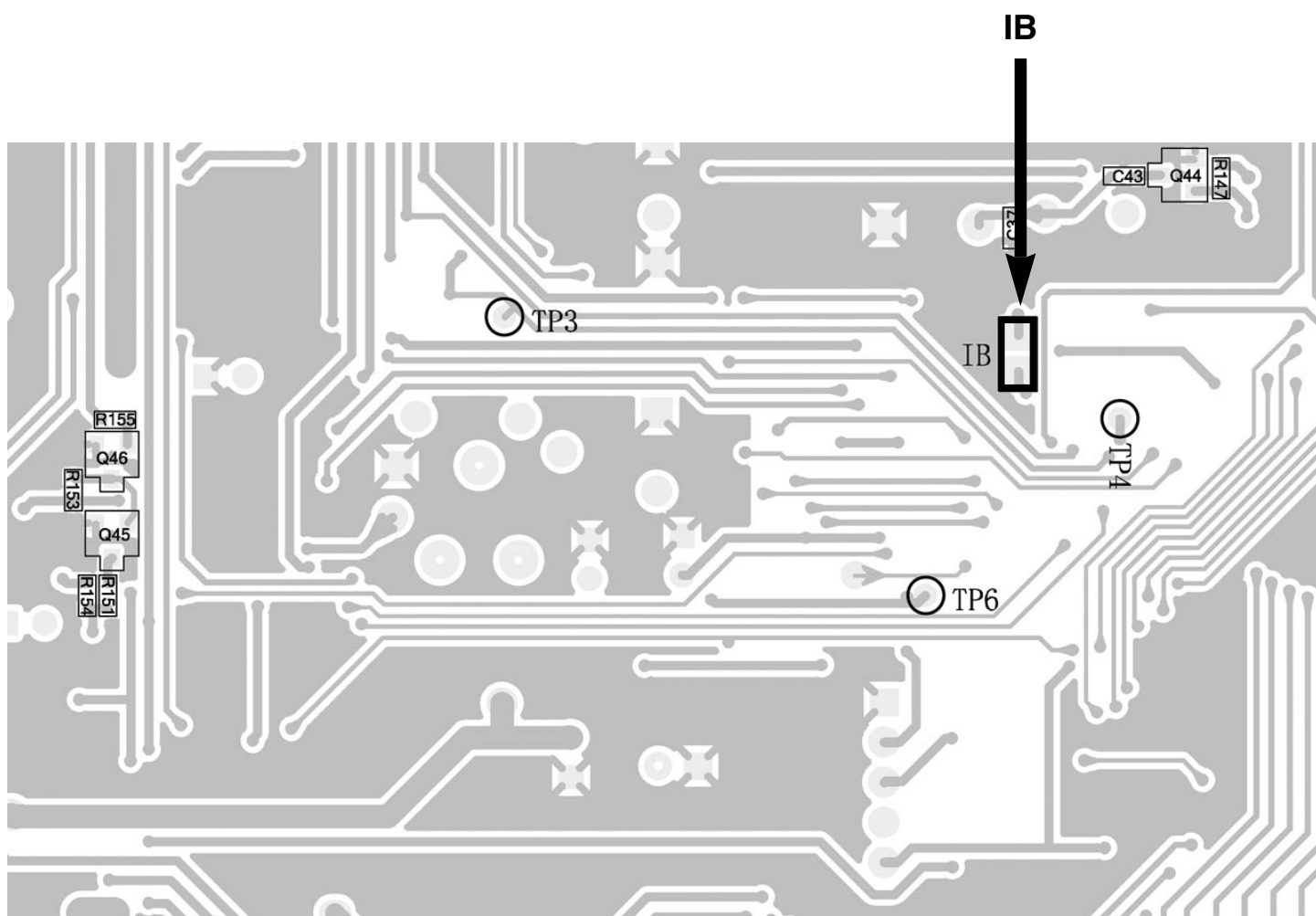
PCB MAIN BOARD BOTTOM
