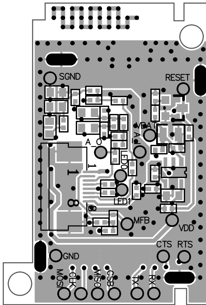
Mechanical Layer
