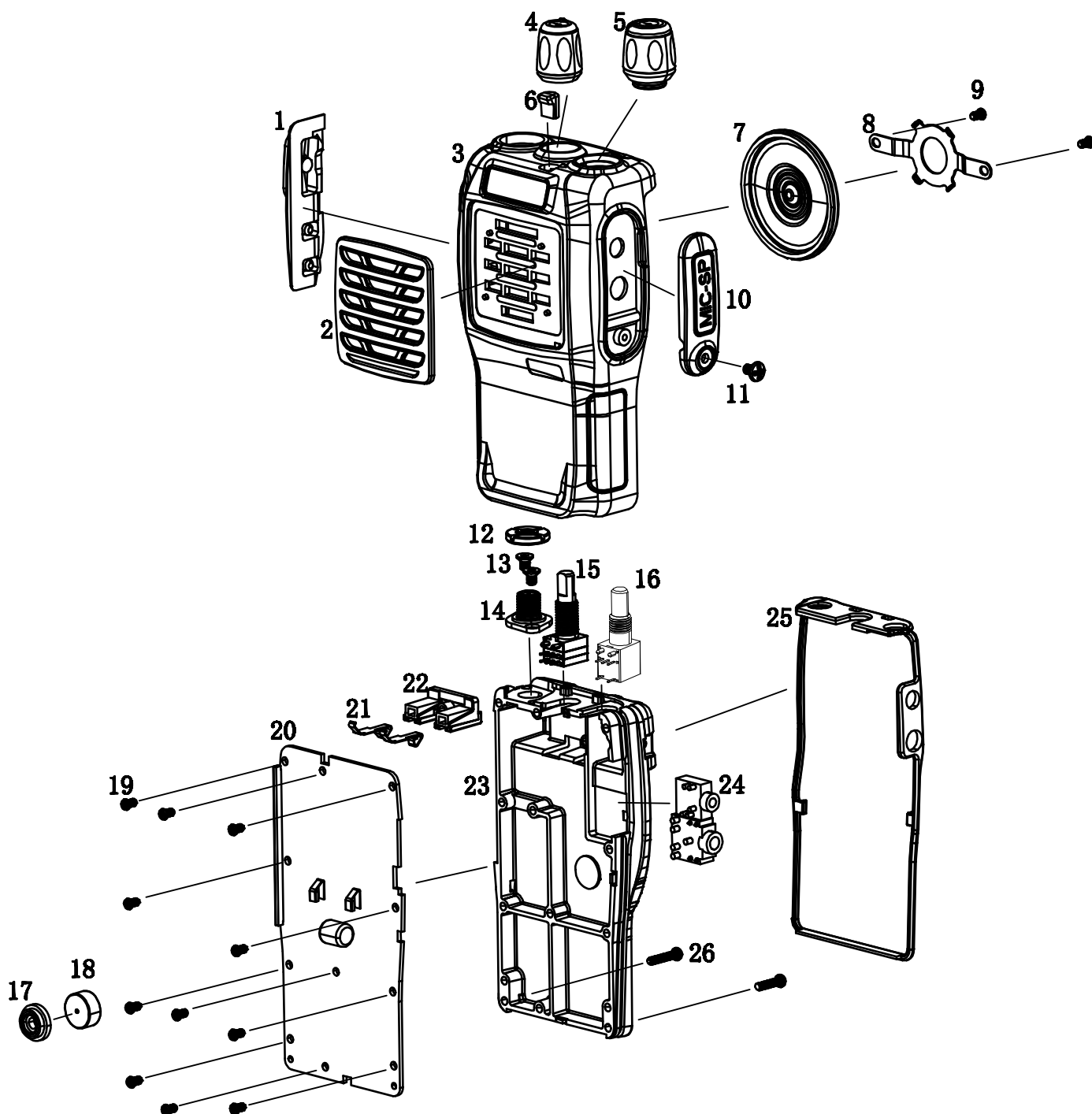
1.PTT key 2.Ornament 3.Housing 4.Channel knob 5.Volume knob 6.Led leader 7.Sperker 8.Speaker mounting bracket 9. Housing screw 10. Earphone cover 11. Earphone screw cover 12. Antenna copper nut 13. Housing screw 14. Antenna Connector 15. Channel Switch 17. MIC set 18. MIC 19. Lock board screw 20. Keypad board 21. Contacts 22. Positive and negative support 23. Aluminum Chassis 24. Earphone seat 25. Aluminum shell waterproof circle 26. Housing screw
