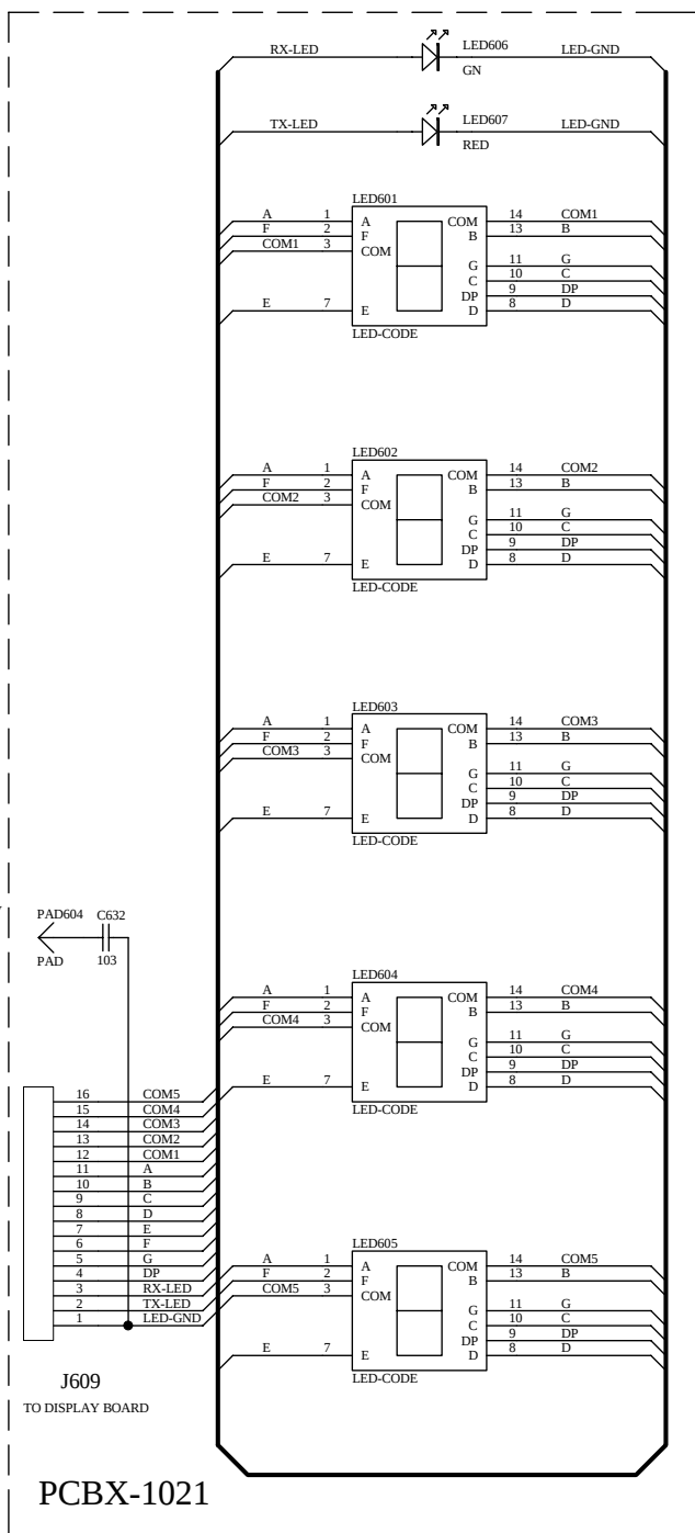
MIDLAND-8001XT Control Board Schematic Diagram
