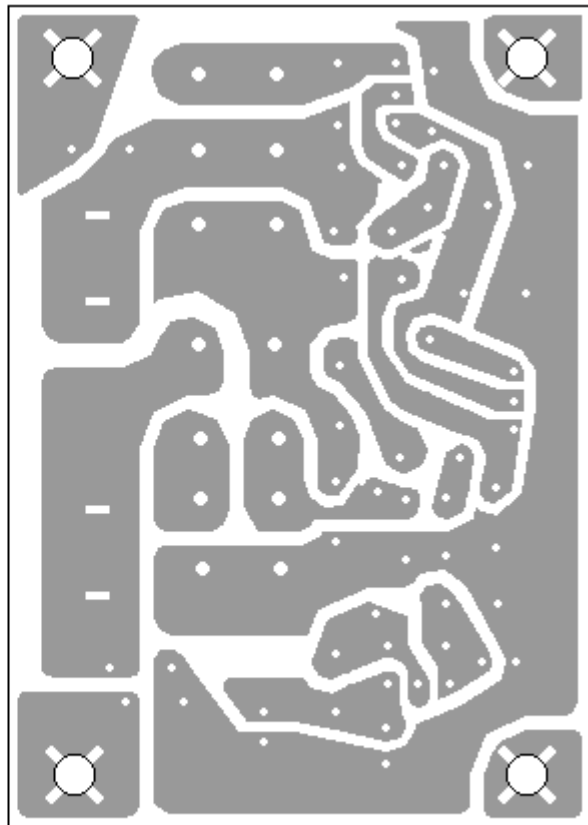
Galaxy DX Radios DX2517 Power Supply PCB EPT0SSB62A
