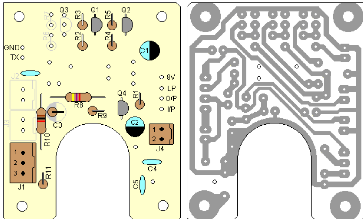
Galaxy DX Radios DX2517 Dimmer PCB EPT55V-51Z
