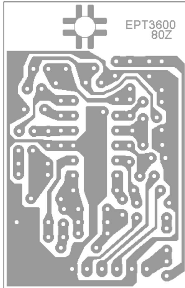
Galaxy DX Radios DX2517 ANF PCB EPT360080Z
